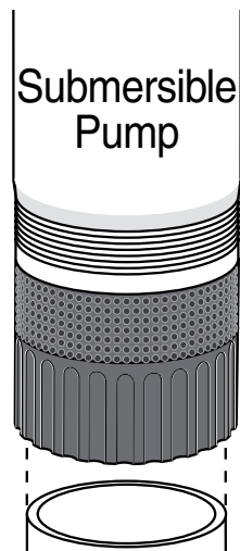
Figure 1: Insert a 3" PVC pipe in the bottom of the motor to raise the pump in the tank.
